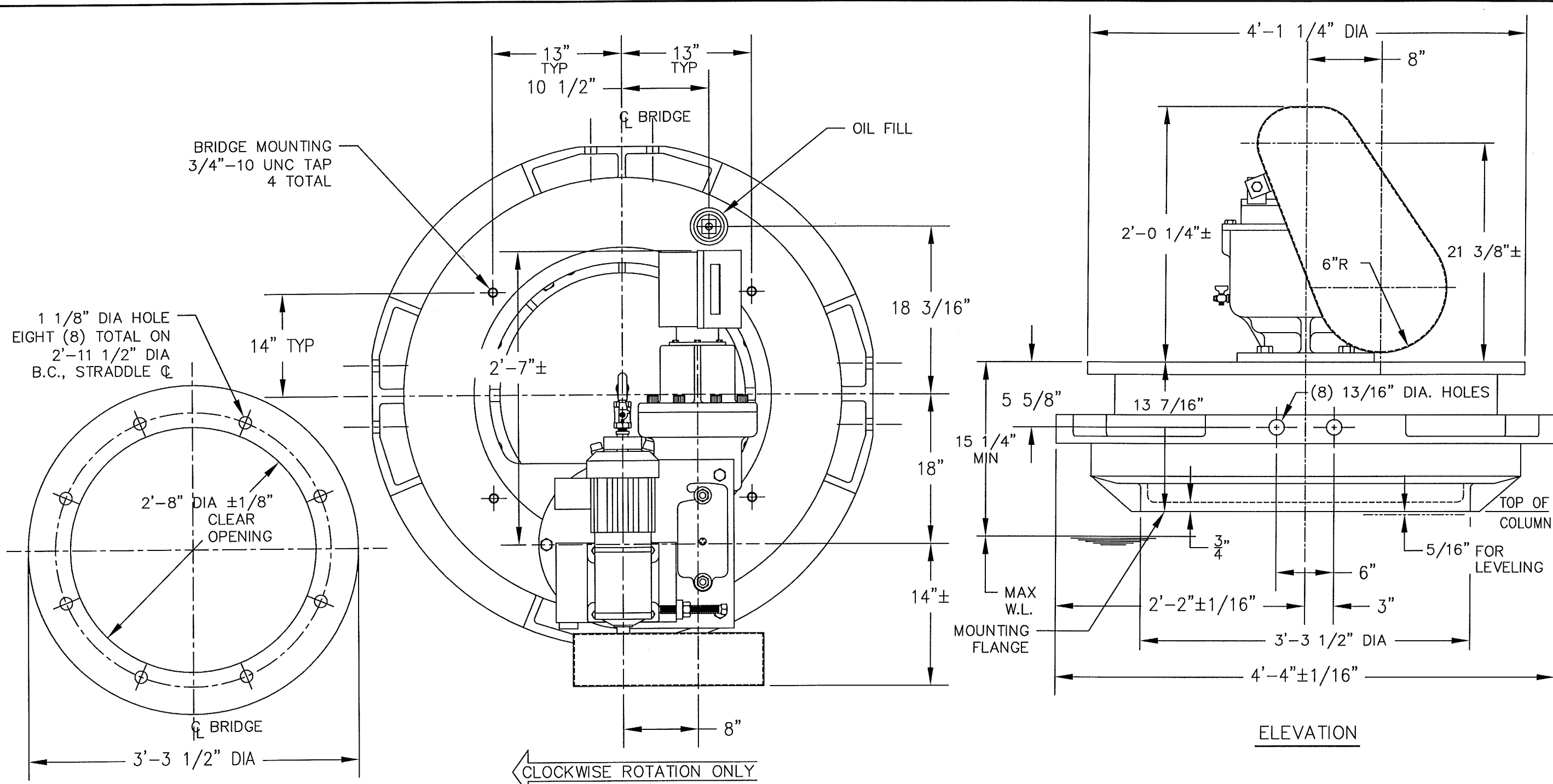
MOUNTING FLANGE
